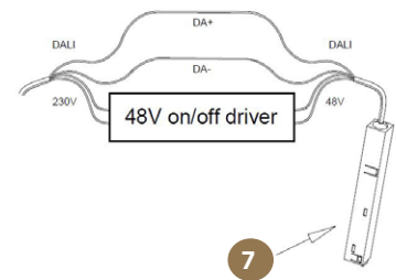
POWER FEED CONNECTION
